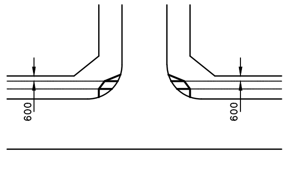
DIAGRAM SHOWING LOCATION OF PEDESTRIAN RAMPS AT INTERSECTIONS
